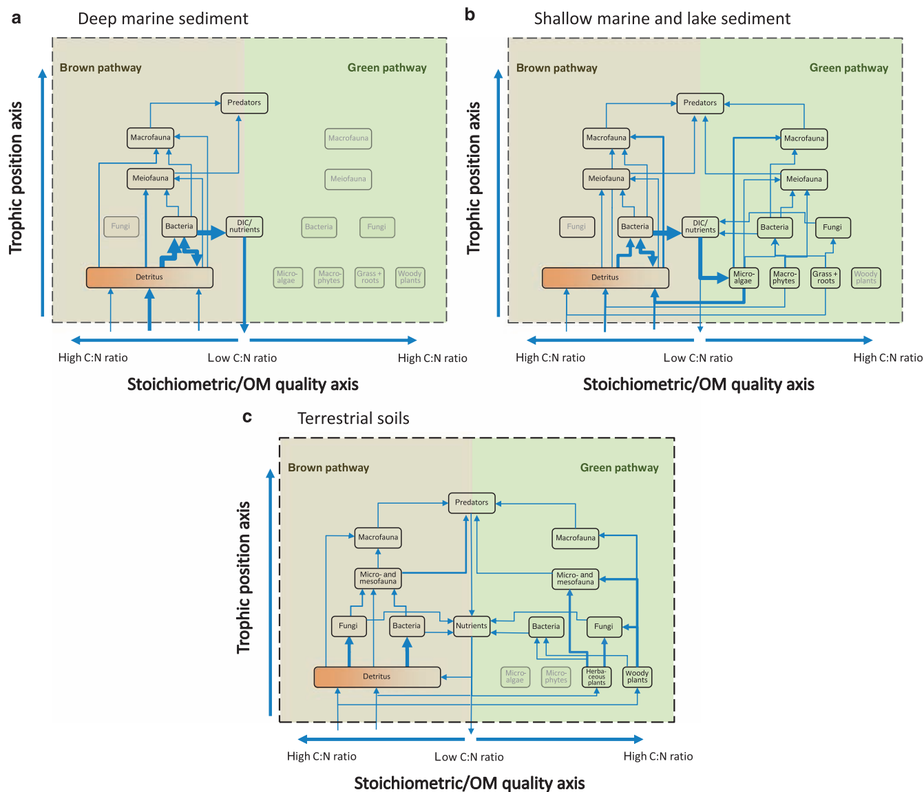
Figure 1. Trophic structure in subsurface food webs as a function of organic matter (OM) quality, including material and interaction flows through both green (right side) and brown (left side) pathways. The arrow weight in the figure indicates the relative importance of material flow and interaction in (a) the deep marine sediment habitats, (b) shallow marine or lake sediment habitats, and (c) terrestrial soil habitats. The arrows entering and leaving detritus reflect their relative position along the stoichiometric quality scale. Although they are depicted as separate boxes, the brown and the green pathways are not separate; there is a high degree of linkage between the two, and they are drawn separately only to convey the concept visually. Furthermore, we show arrows from dead photosynthetic production to the detrital pool, because this is the primary source of biomass flux there. Although the arrows connecting higher trophic levels with detritus were excluded, we do not want to ignore their contributions, but we leave them out for clarity of presentation. Abbreviations: C, carbon; DIC, dissolved inorganic carbon; N, nitrogen.
